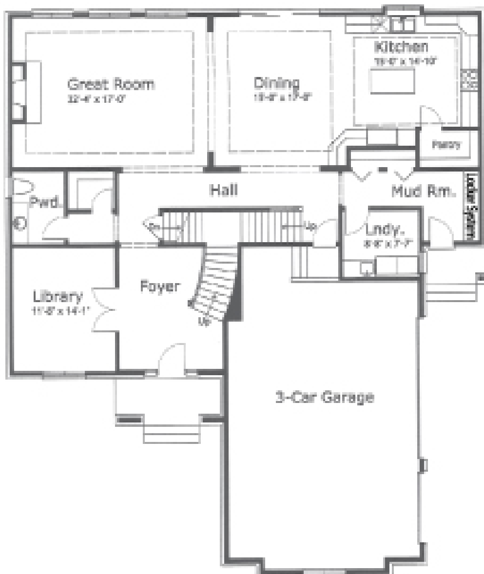
FIRST FLOOR PLAN 3,700 Approx. sq. ft. Total
